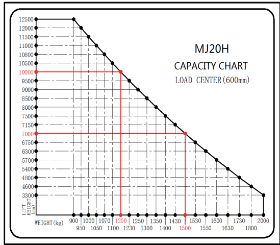
Capacity Chart-MJ20H
