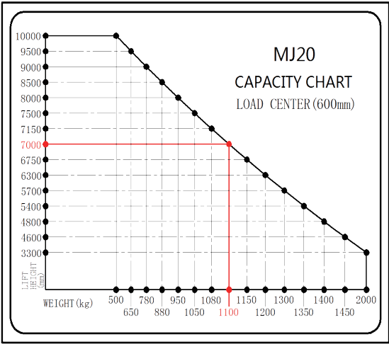
Capacity Chart-MJ20
